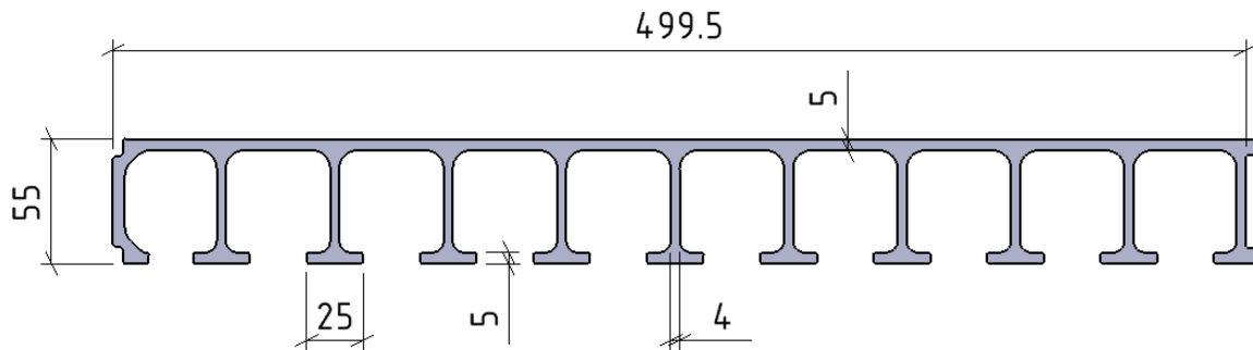
figure 5: Geometry plank 500.55
