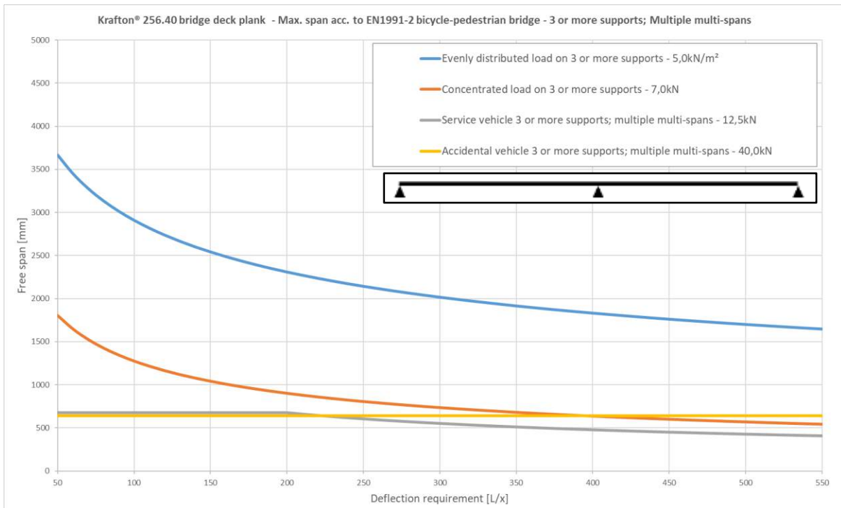
figure 4: Maximum span as a function of deflection requirements; 3 or more supports
