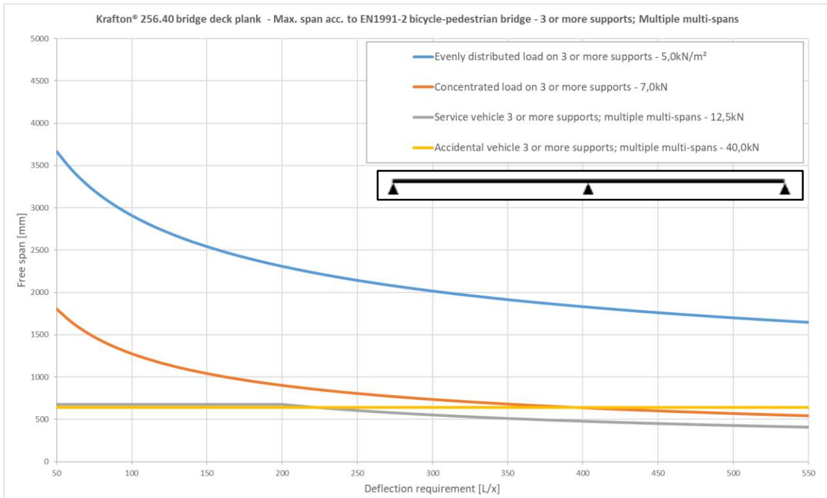
figure 8: Maximum span as a function of deflection requirements; 3 or more supports
